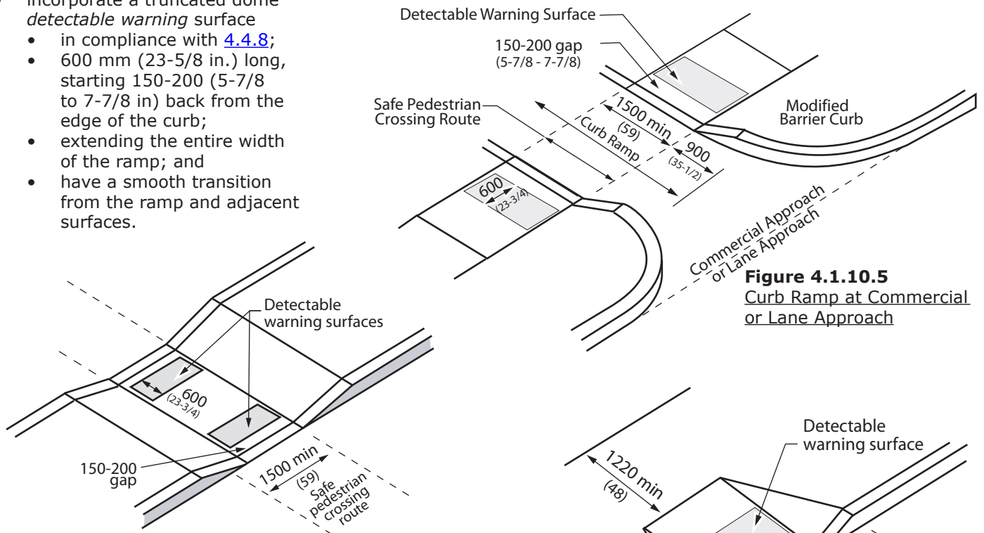
Figure 4.1.10.3 Curb Ramp at Narrow Median Sidewalk Crossing
