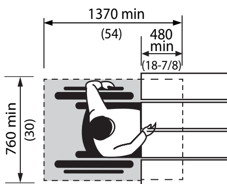
Figure 4.3.7.2 Frontal Approach
