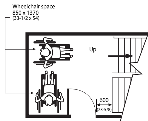
Figure 4.4.1.1 Area of Rescue Assistance
