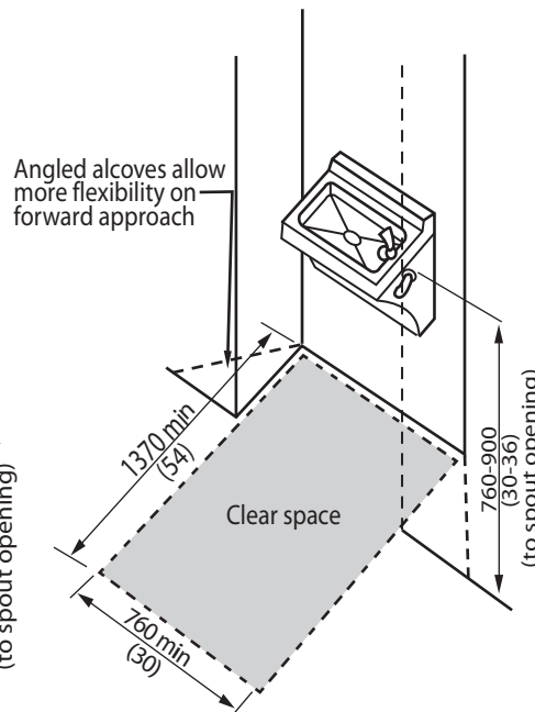
Figure 4.3.1.2 Forward Approach
