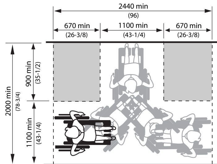
Figure 4.1.1.2 180° Turning Space
