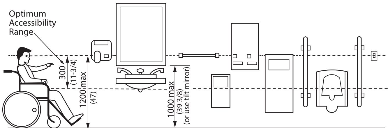
Figure 4.2.6.1 Washroom Accessories
