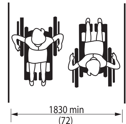
Figure 4.1.4.2 Access Widths
