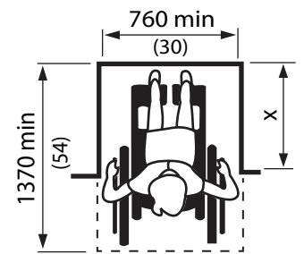
Figure 4.1.1.7 Clearances at Alcove
