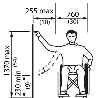
Figure 4.1.1.9 Side Reach
