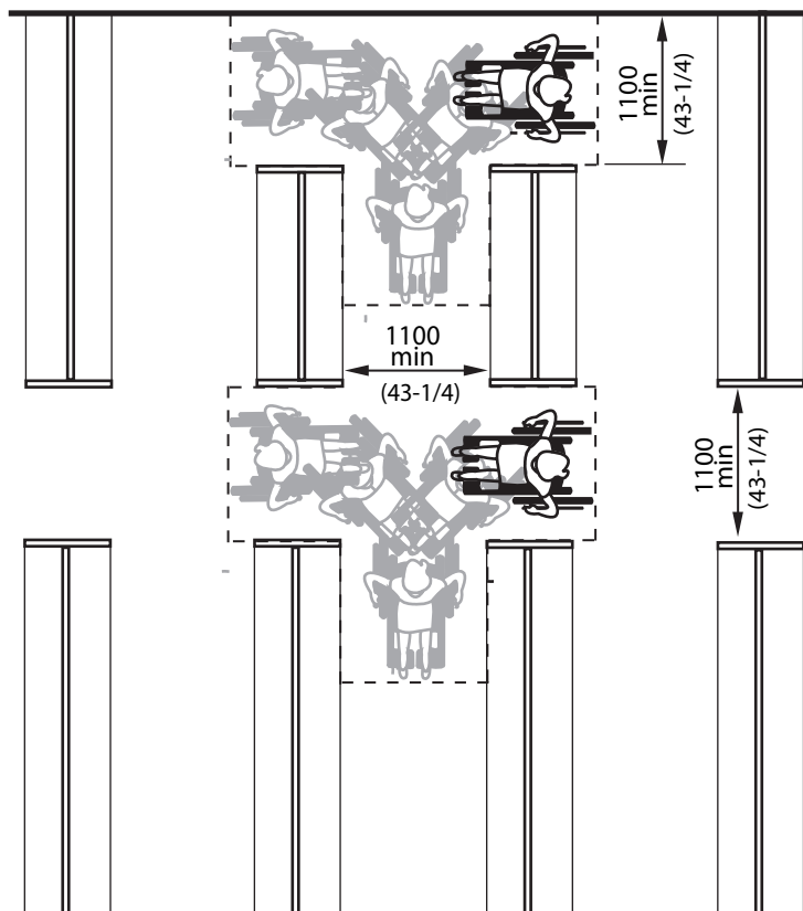
Figure 4.5.6.1 Aisle Width
