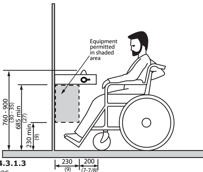
Figure 4.3.1.2 Forward Approach
