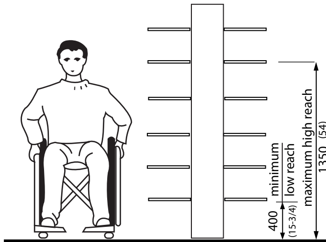
Figure 4.5.6.2 Reach Heights
