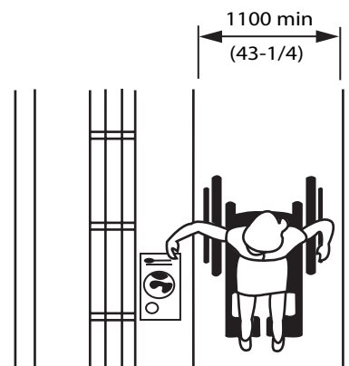
Figure 4.5.4.2 Aisle Width
