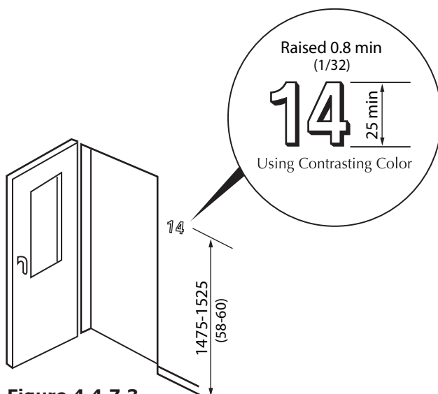
Figure 4.4.7.3 Tactile Lettering
