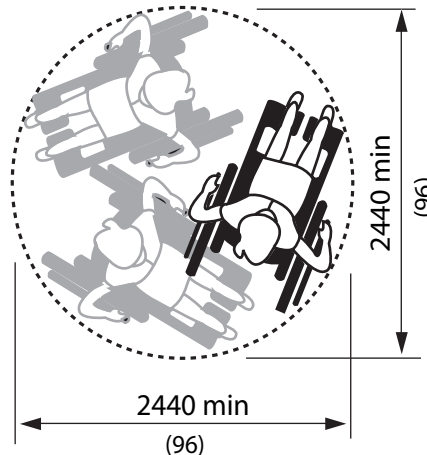
Figure 4.1.1.1 360° Turning Space
