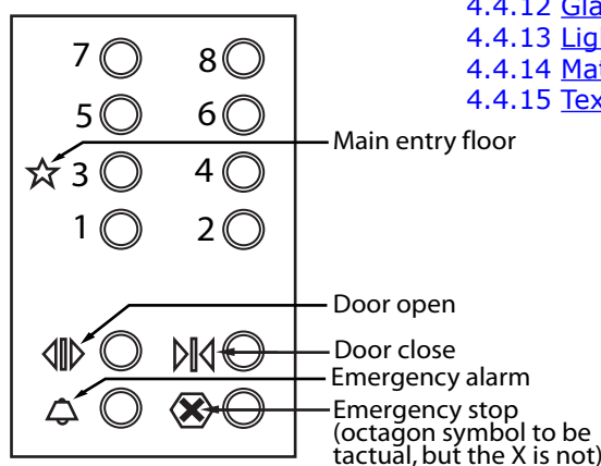
Figure 4.1.14.4 Tactile Symbols
