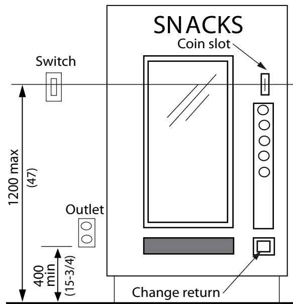
Figure 4.4.3.1 Vending Machine
