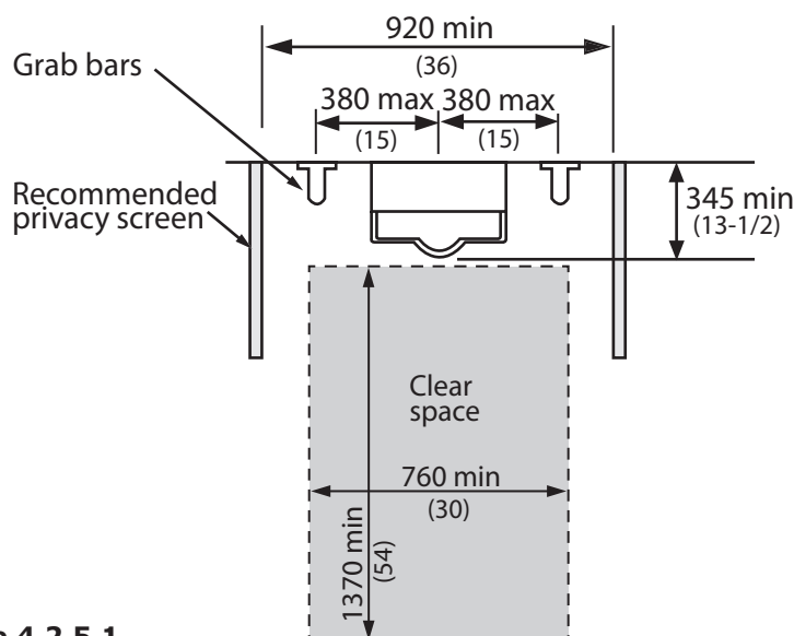
Figure 4.2.5.1 Urinal
