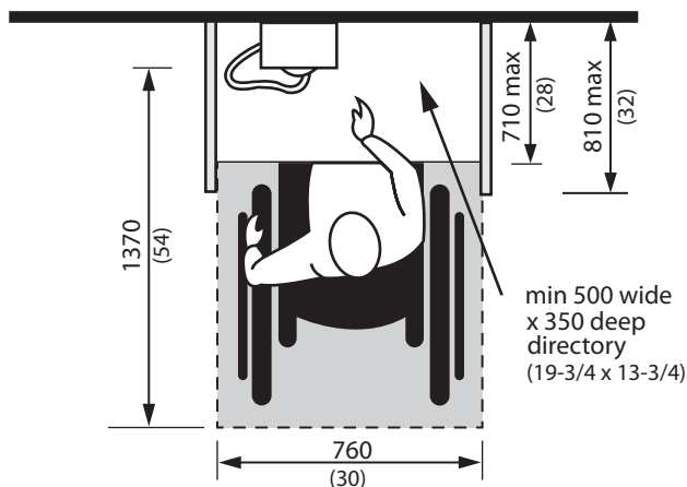
Figure 4.4.5.3 Parallel Approach to a Public Telephone
