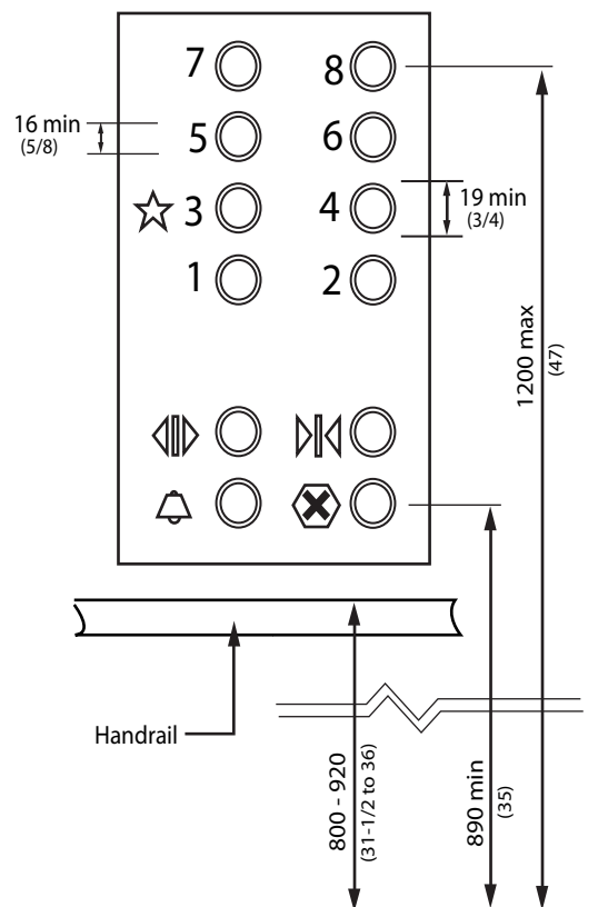
Figure 4.1.14.2 Control Panel
