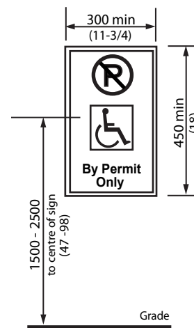
Figure 4.3.12.3 Designated Parking Signage
