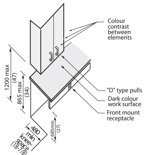
Figure 4.3.18.4 Storage Elements
