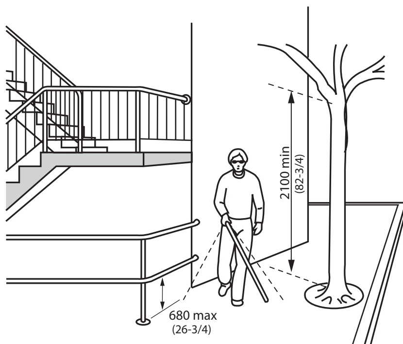
Figure 4.1.3.3 Overhead Obstructions
